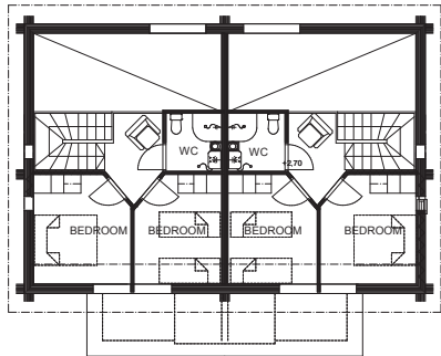
Fjell top cottages, 2nd floor
