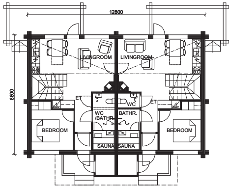
Fjell top cottages, 1st floor
